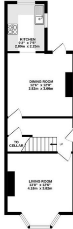
GROUND FLOOR 442 sq.ft. (40.7 sq.m.) approx.
