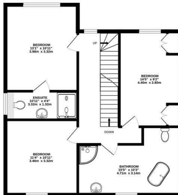
1ST FLOOR 695 sq.ft. (64.5 sq.m.) approx.
