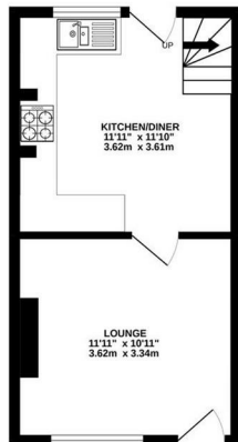
GROUND FLOOR - MAX ROOM HEIGHT = 2.63M
