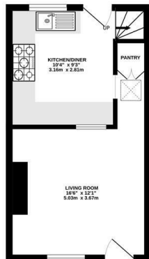
GROUND FLOOR 256 sq.ft. (23.6 sq.m.) approx.
