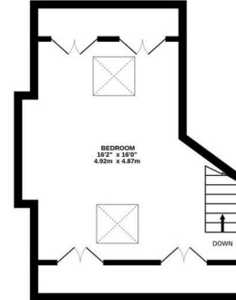
2ND FLOOR 275 sq.ft. (25.5 sq.m.) approx.
